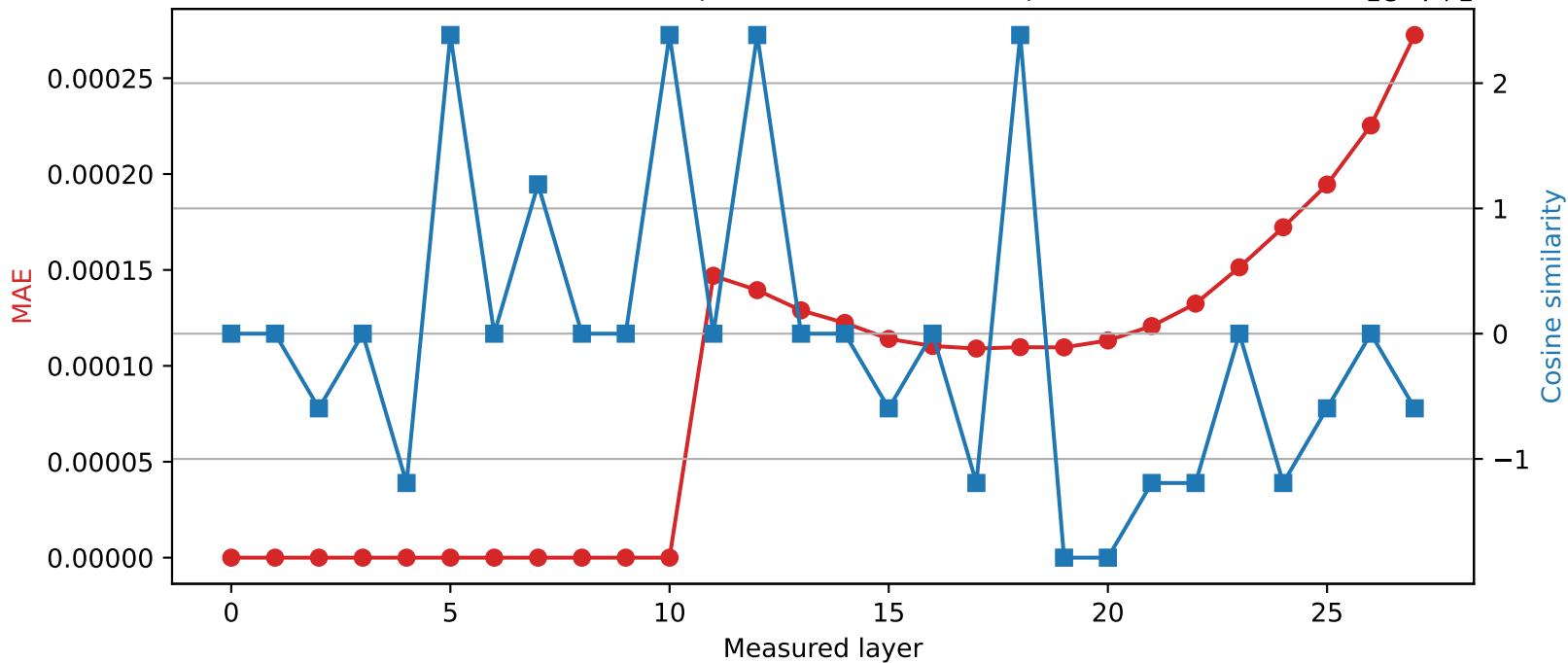
Qwen2.5-7B-Instruct | Quantized layer 10 | float64 → int16
