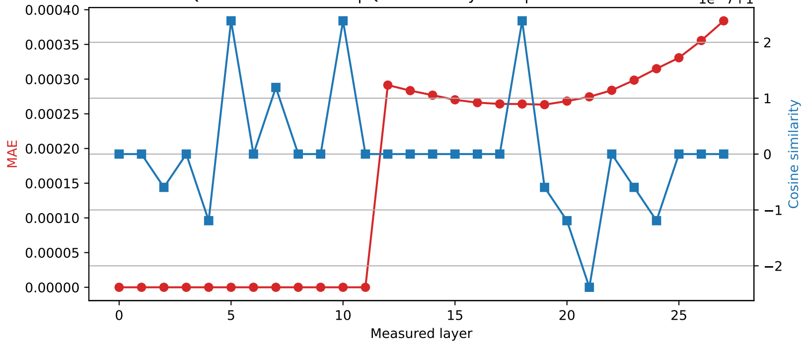
Qwen2.5-7B-Instruct | Quantized layer 11 | float64 → int16
