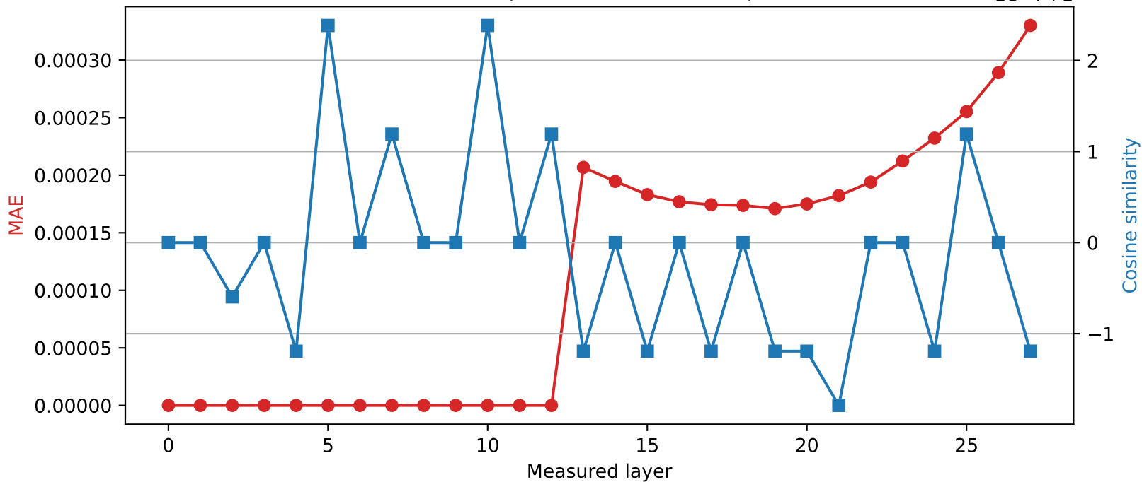
Qwen2.5-7B-Instruct | Quantized layer 12 | float64 → int16
