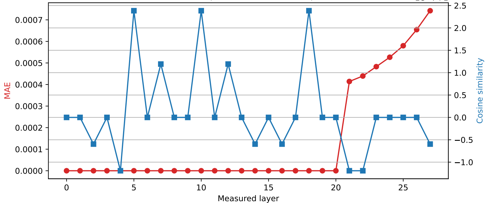
Qwen2.5-7B-Instruct | Quantized layer 20 | float64 \rightarrow int16
