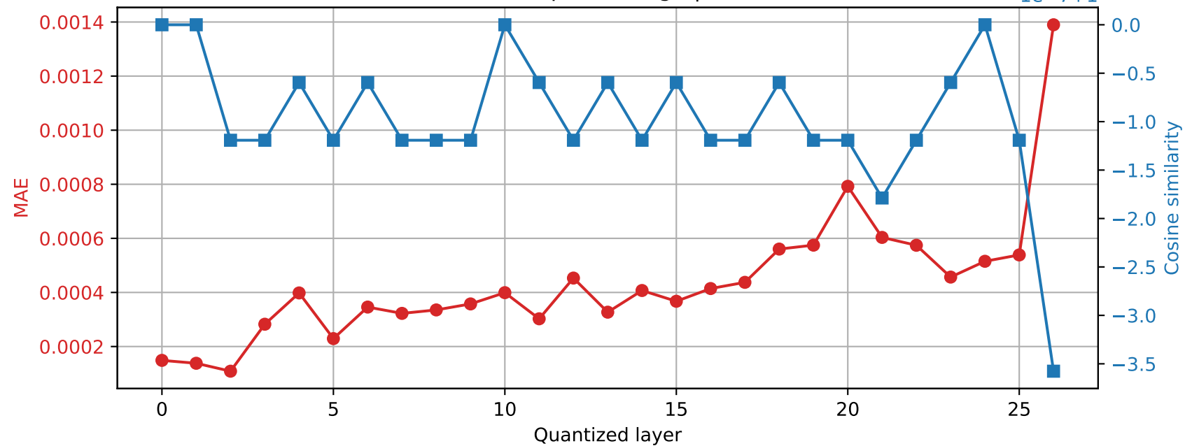
Qwen2.5-7B-Instruct | Prompt 1 Final RMSNorm output damage | float64 → int16
