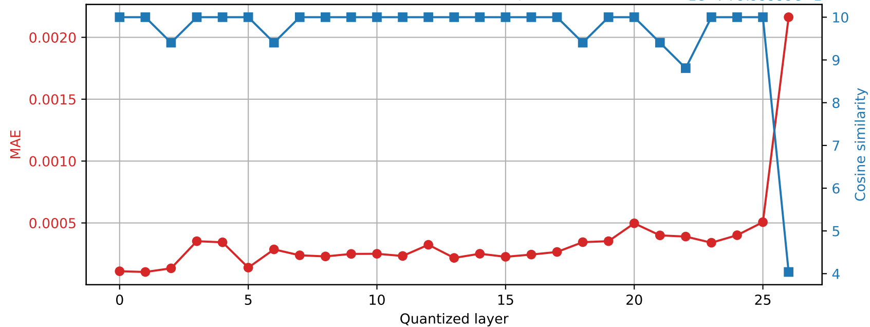
Qwen2.5-7B-Instruct | Prompt 2 Final RMSNorm output damage | float64 → int16
