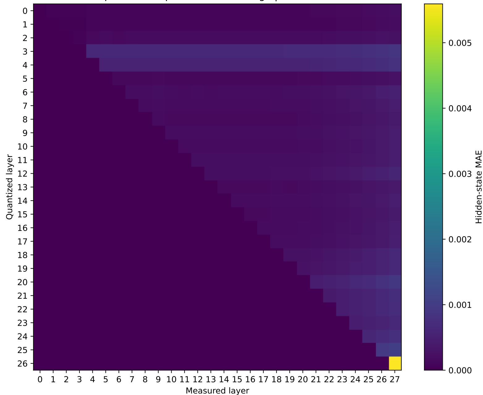
Qwen2.5-7B-Instruct Prompt 2: MAE representation damage | float64 → int16
