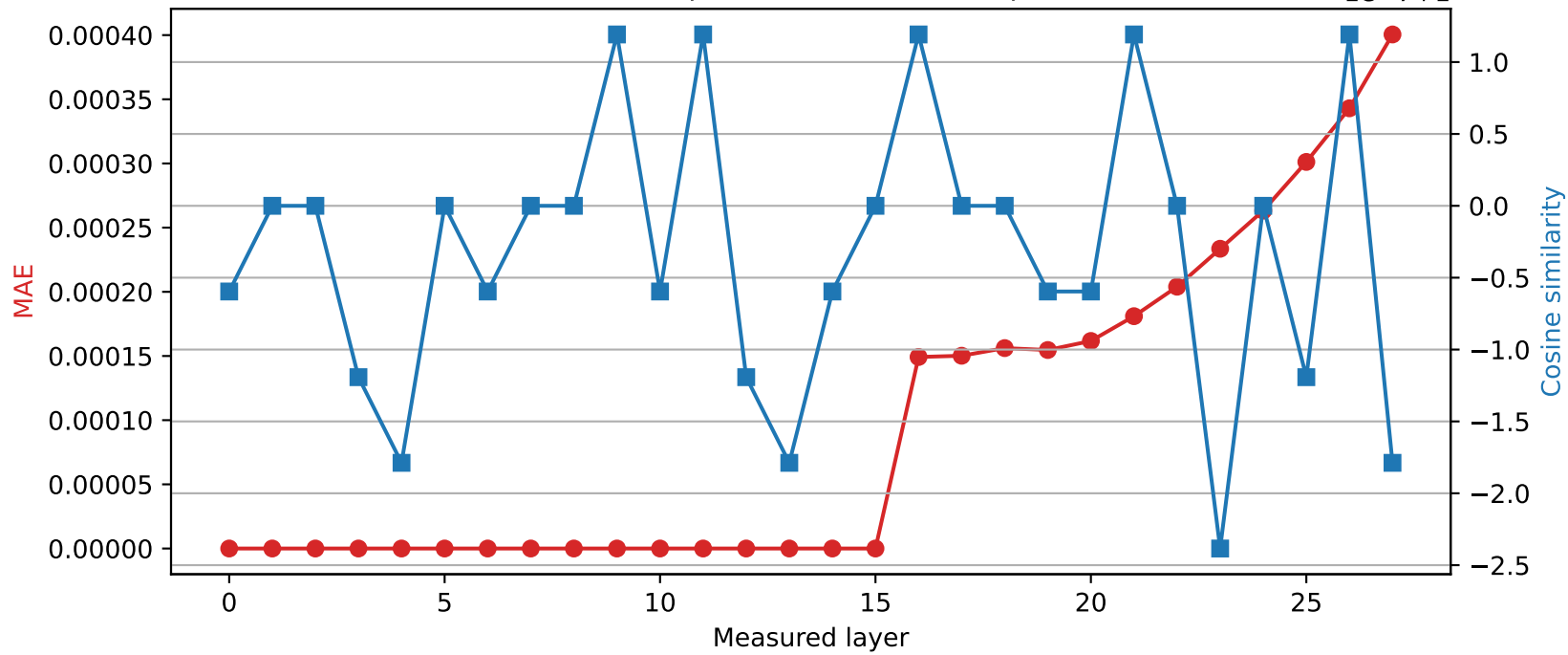
Qwen2.5-7B-Instruct | Quantized layer 15 | float64 → int16
