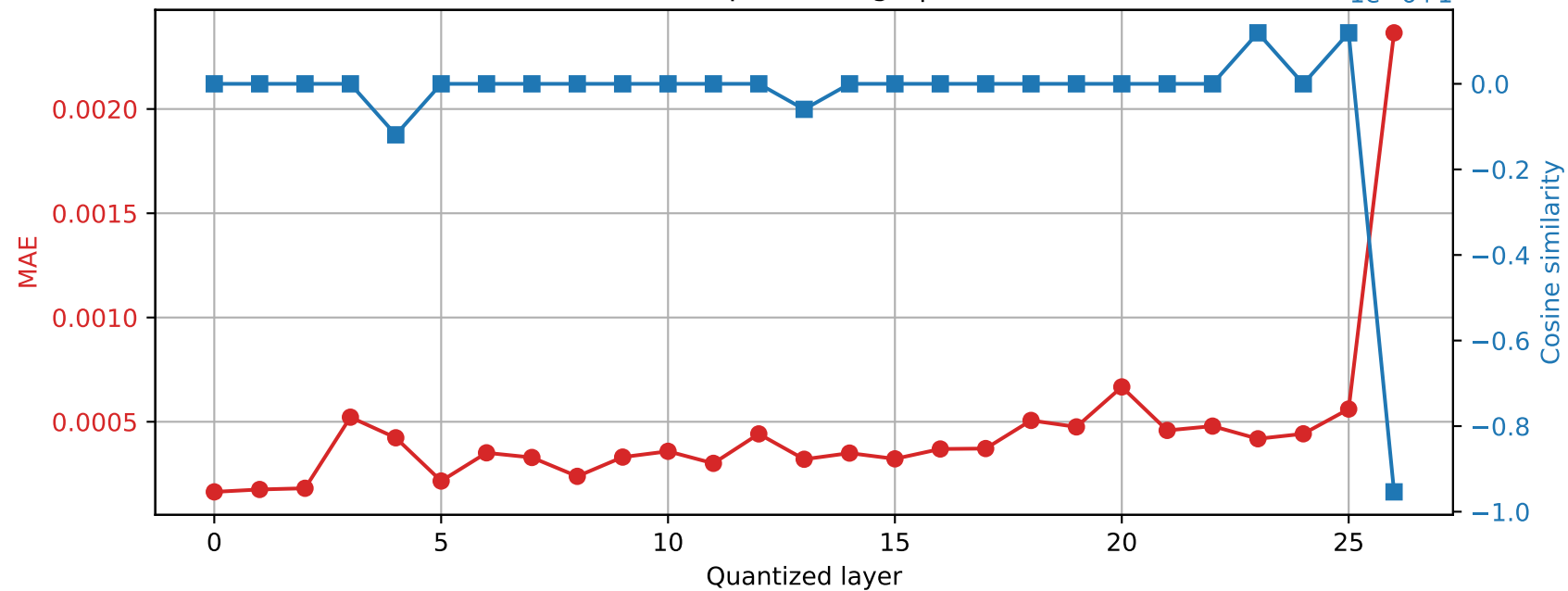
Qwen2.5-7B-Instruct | Prompt 3 Final RMSNorm output damage | float64 → int16
