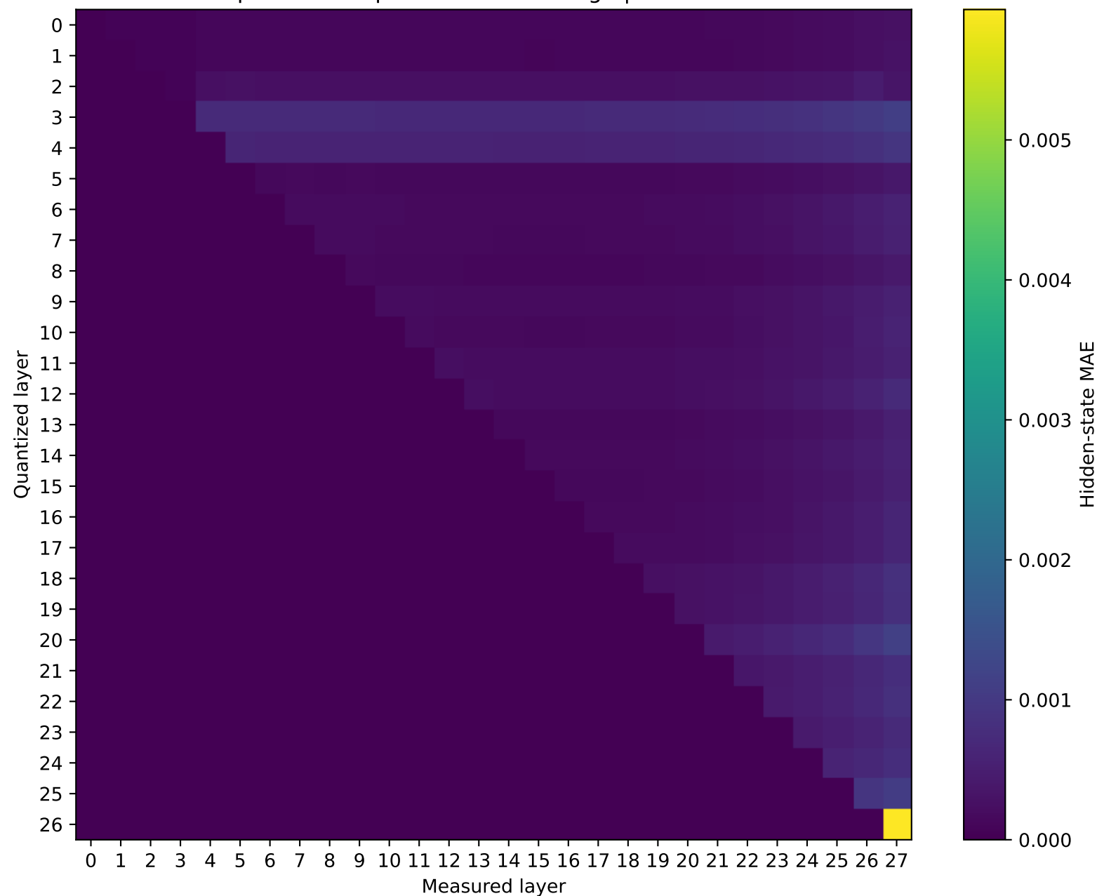
Qwen2.5-7B-Instruct Prompt 3: MAE representation damage | float64 → int16
