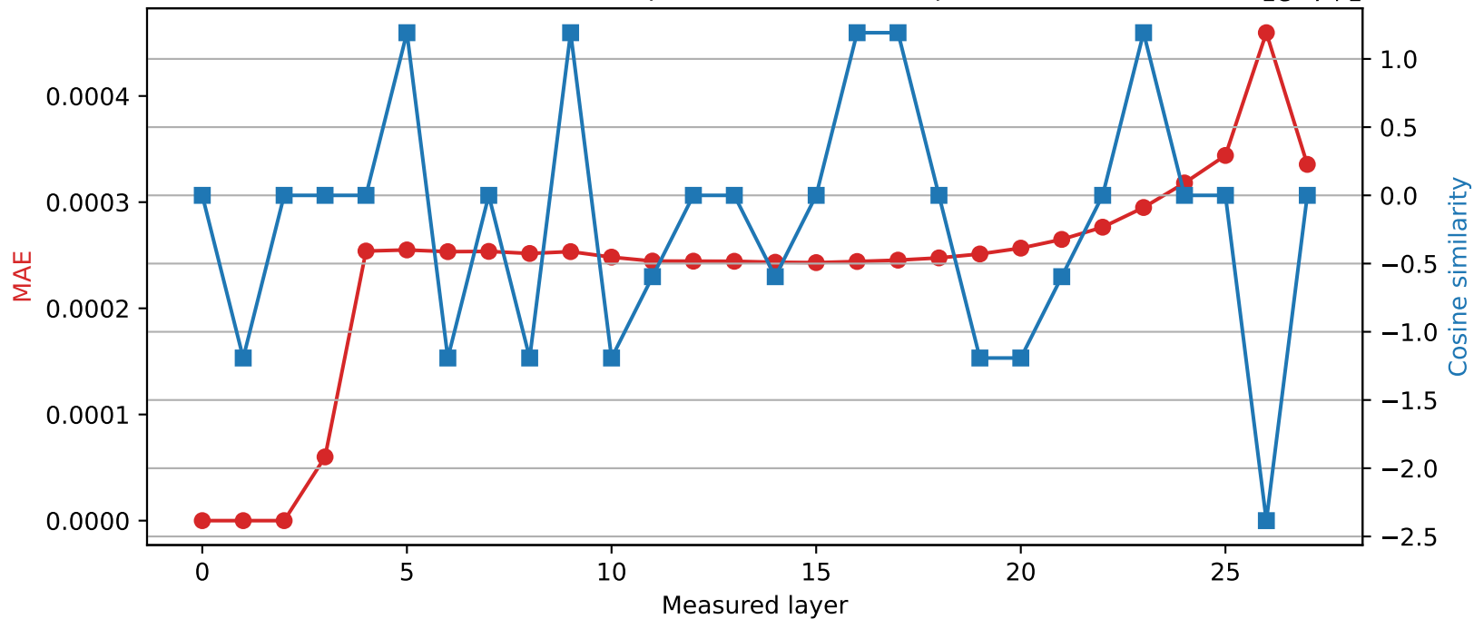
Qwen2.5-7B-Instruct | Quantized layer 2 | float64 → int16
