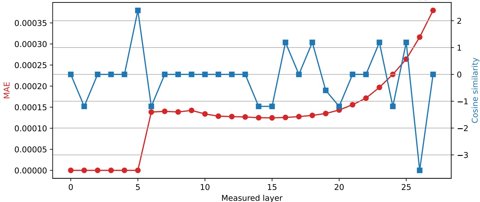
Qwen2.5-7B-Instruct | Quantized layer 5 | float64 → int16
