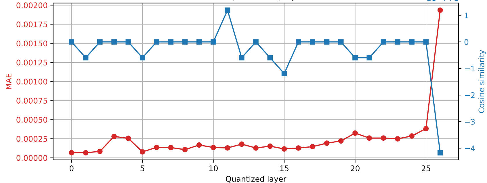
Qwen2.5-7B-Instruct | Prompt 4 Final RMSNorm output damage | float64 → int16
