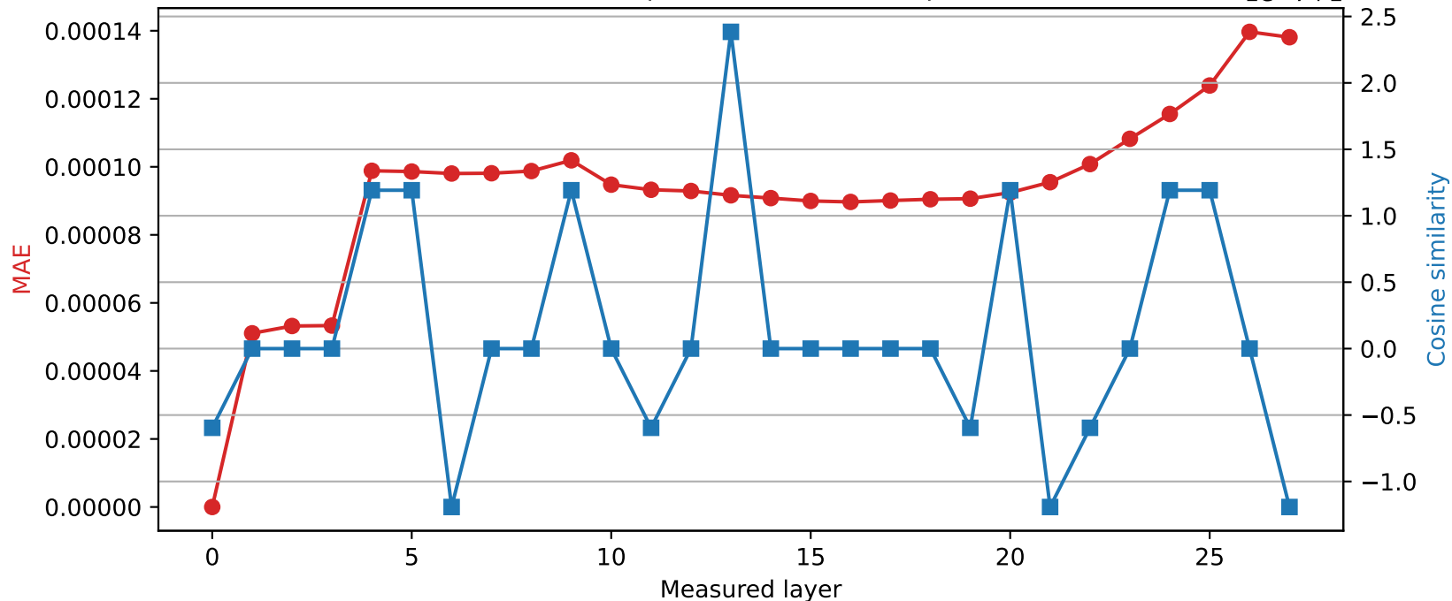
Qwen2.5-7B-Instruct | Quantized layer 0 | float64 → int16
