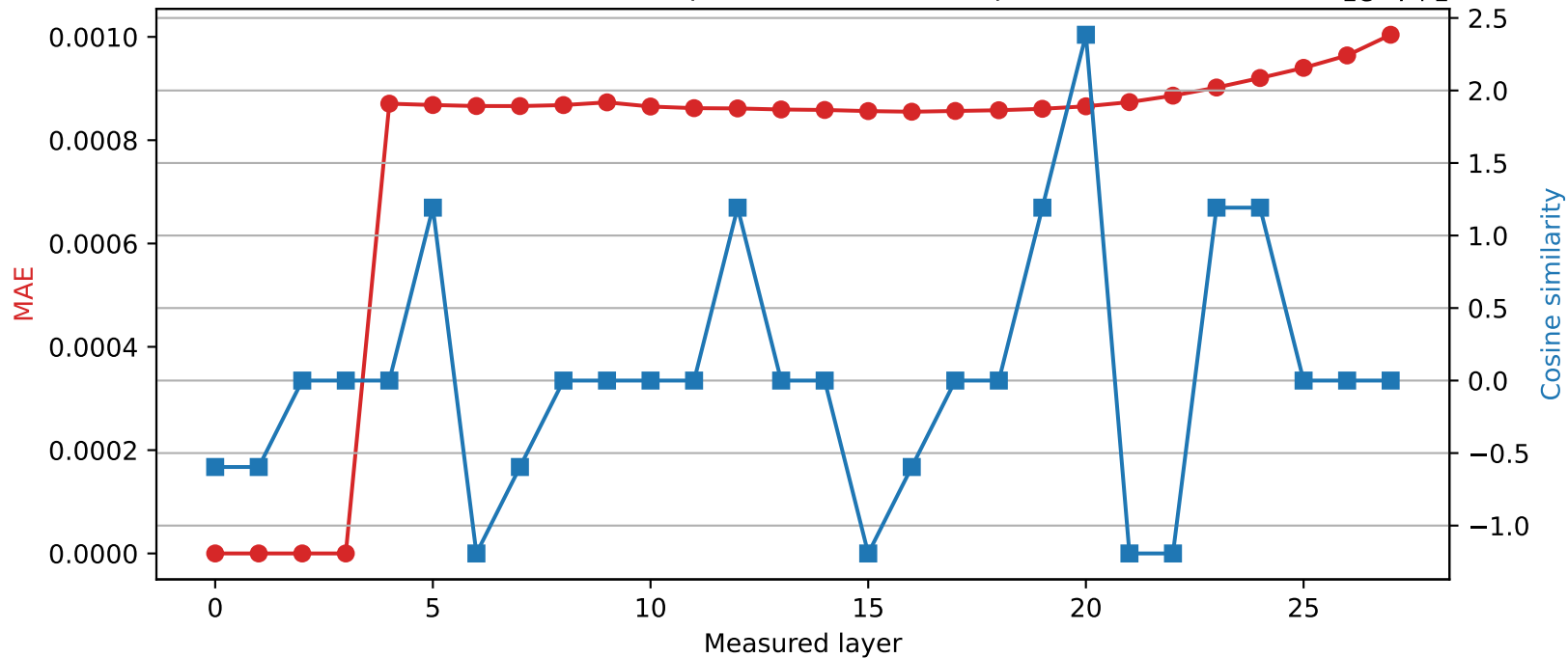
Qwen2.5-7B-Instruct | Quantized layer 3 | float64 → int16
