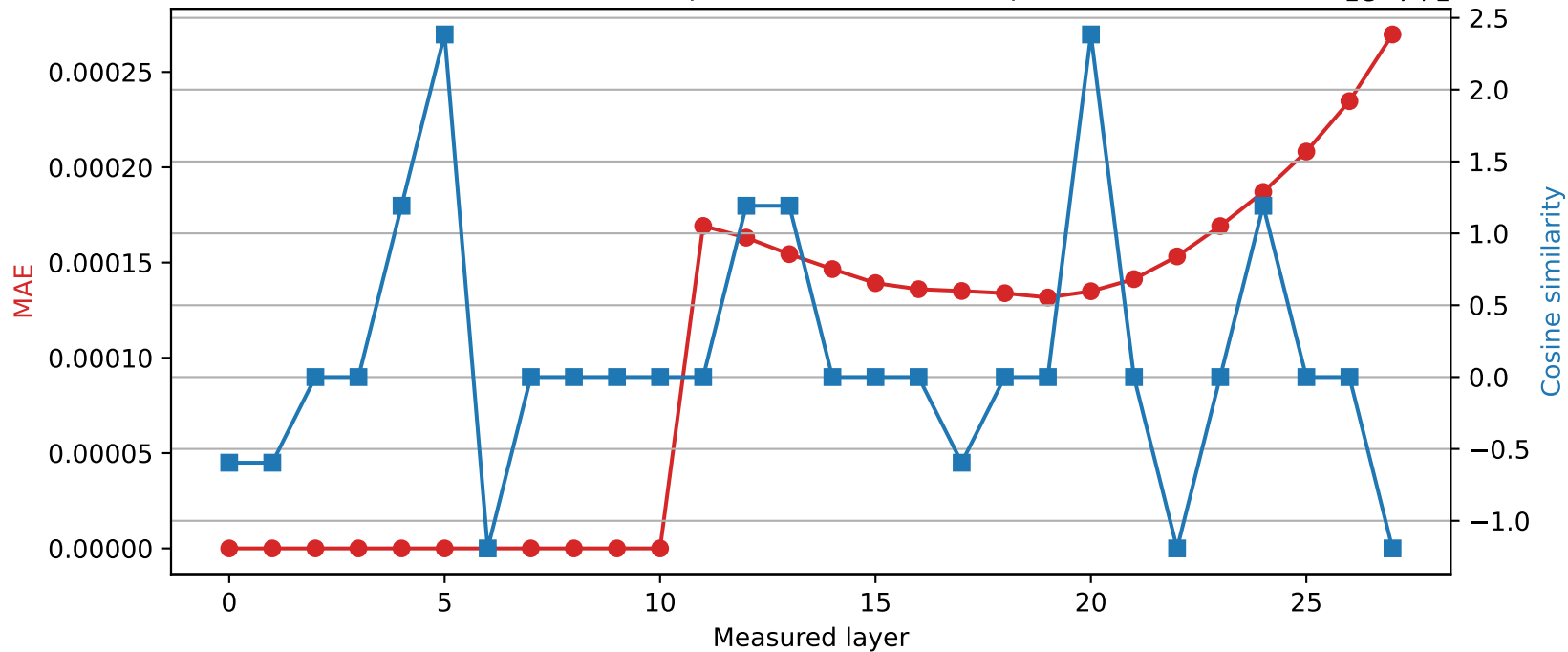
Qwen2.5-7B-Instruct | Quantized layer 10 | float64 \rightarrow int16
