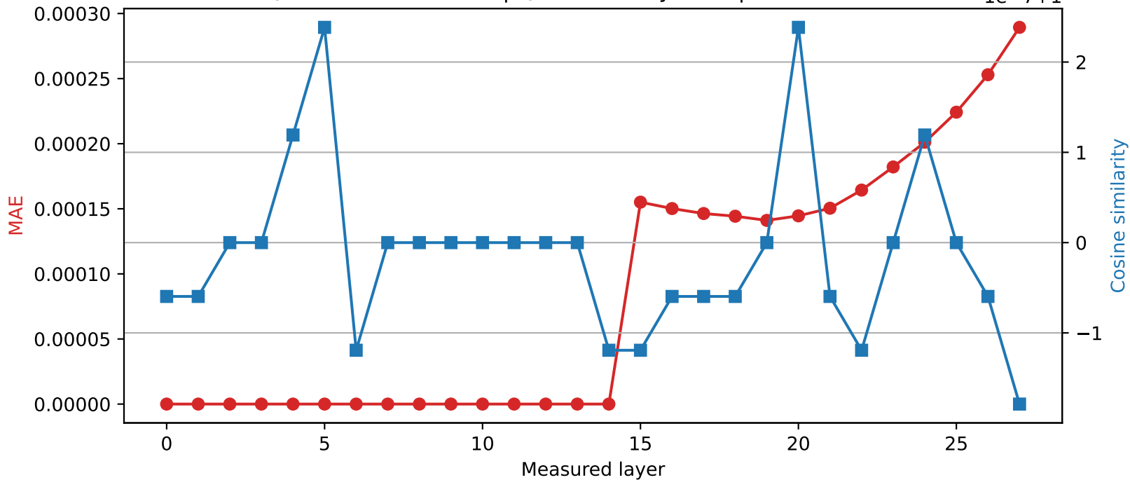
Qwen2.5-7B-Instruct | Quantized layer 14 | float64 → int16
