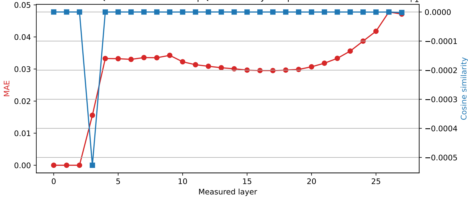
Qwen2.5-7B-Instruct | Quantized layer 2 | float64 → int8
