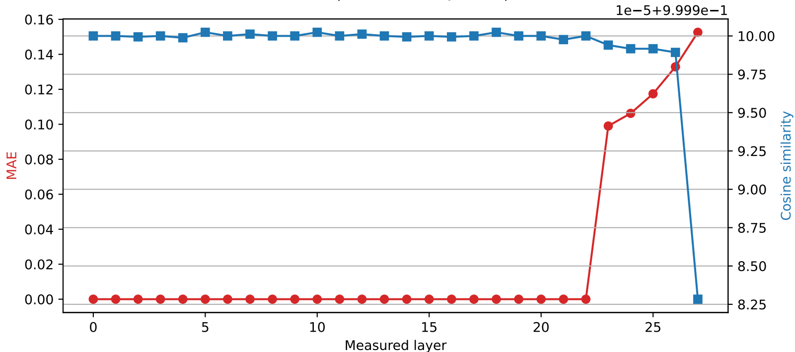
Qwen2.5-7B-Instruct | Quantized layer 22 | float64 → int8
