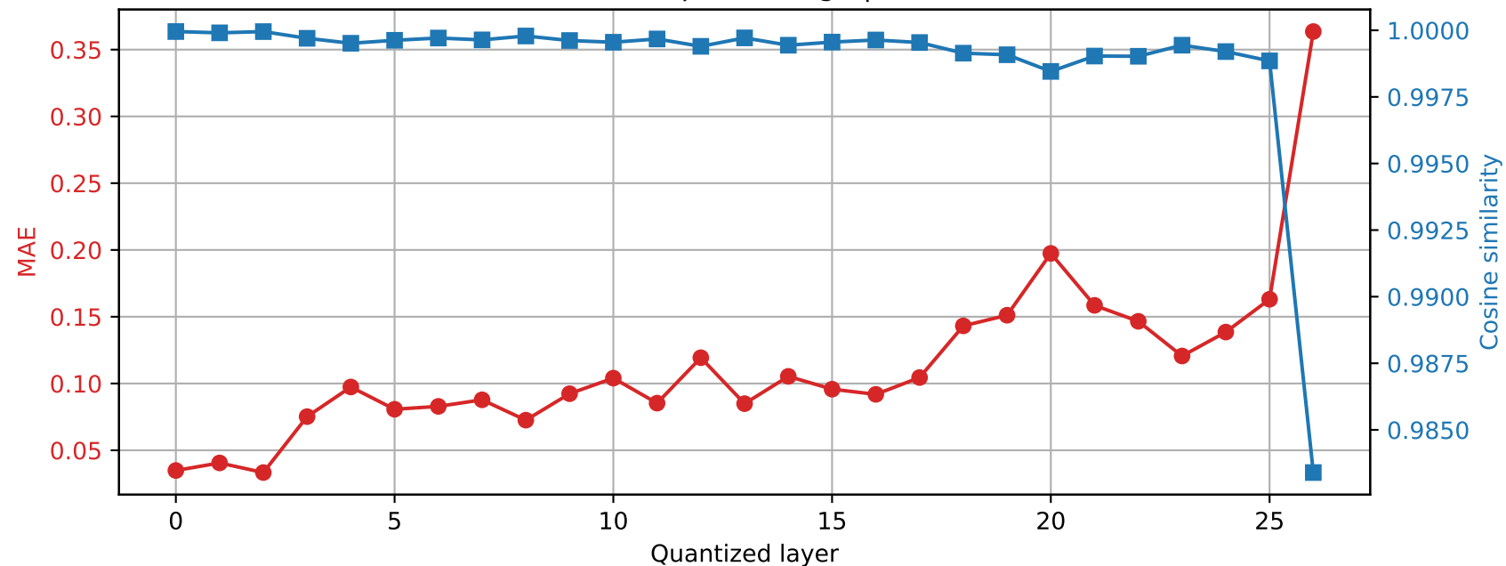
Qwen2.5-7B-Instruct | Prompt 1 Final RMSNorm output damage | float64 → int8
