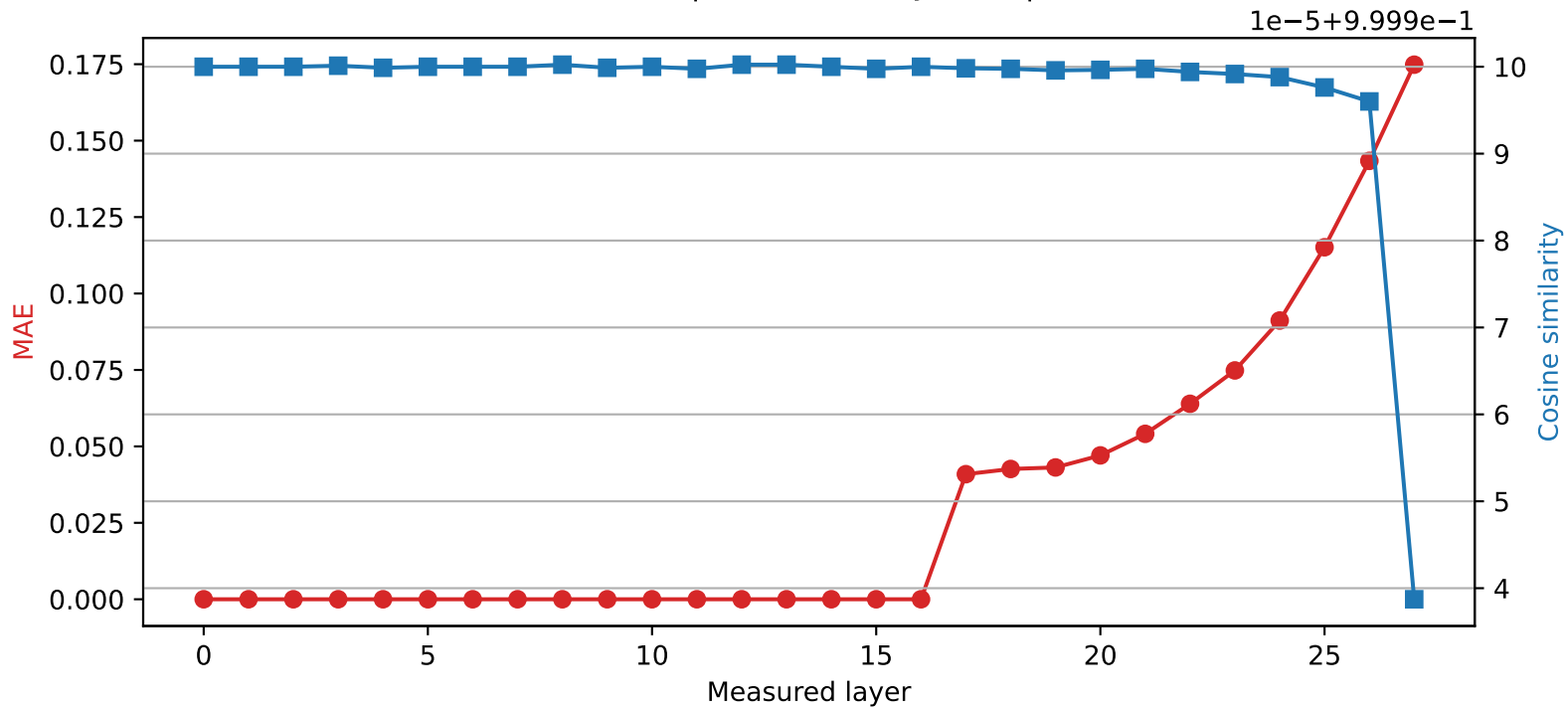
Qwen2.5-7B-Instruct | Quantized layer 16 | float64 → int8
