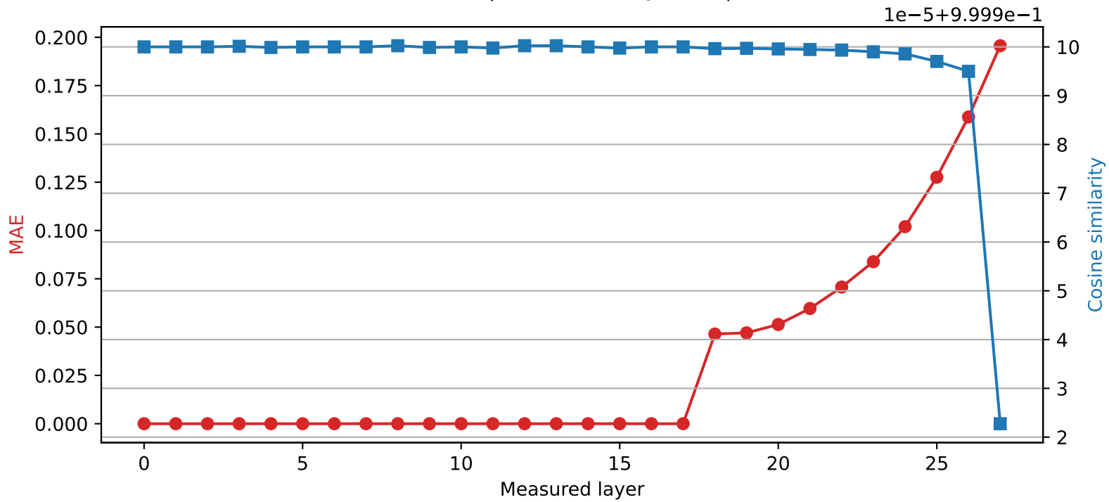
Qwen2.5-7B-Instruct | Quantized layer 17 | float64 \rightarrow int8
