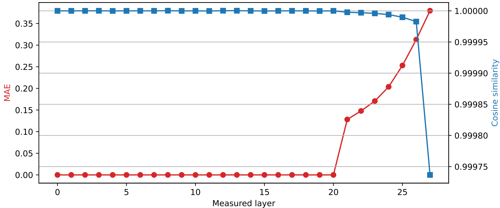
Qwen2.5-7B-Instruct | Quantized layer 20 | float64 \rightarrow int8
