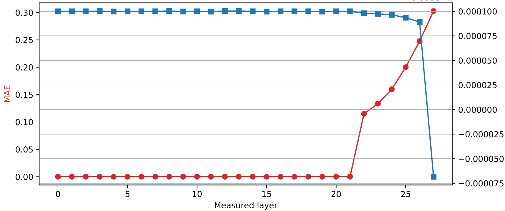
Qwen2.5-7B-Instruct | Quantized layer 21 | float64 \rightarrow int8
