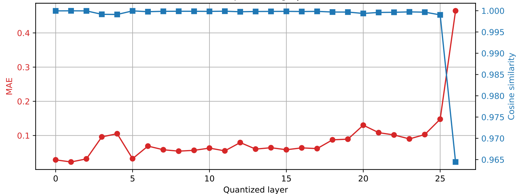
Qwen2.5-7B-Instruct | Prompt 2 Final RMSNorm output damage | float64 \rightarrow int8
