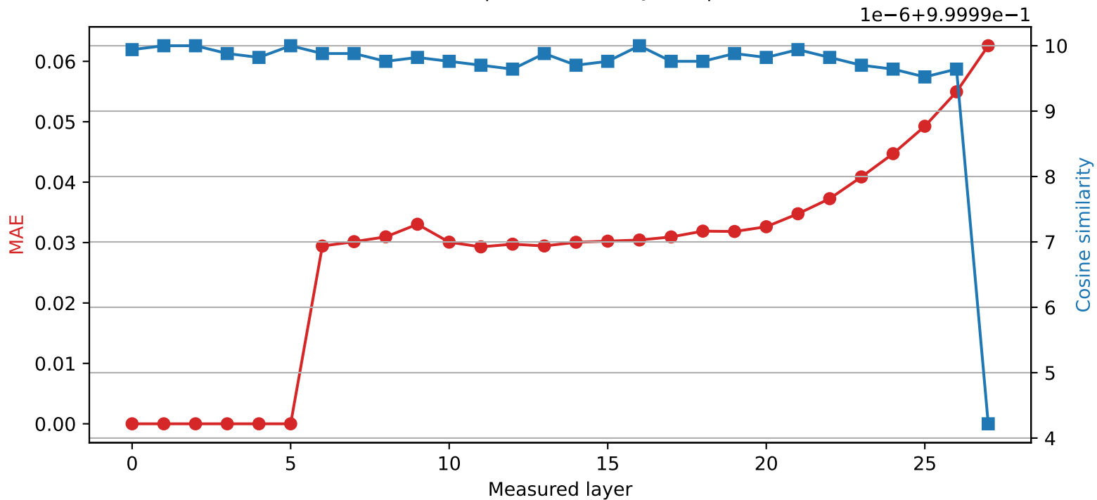
Qwen2.5-7B-Instruct | Quantized layer 5 | float64 → int8
