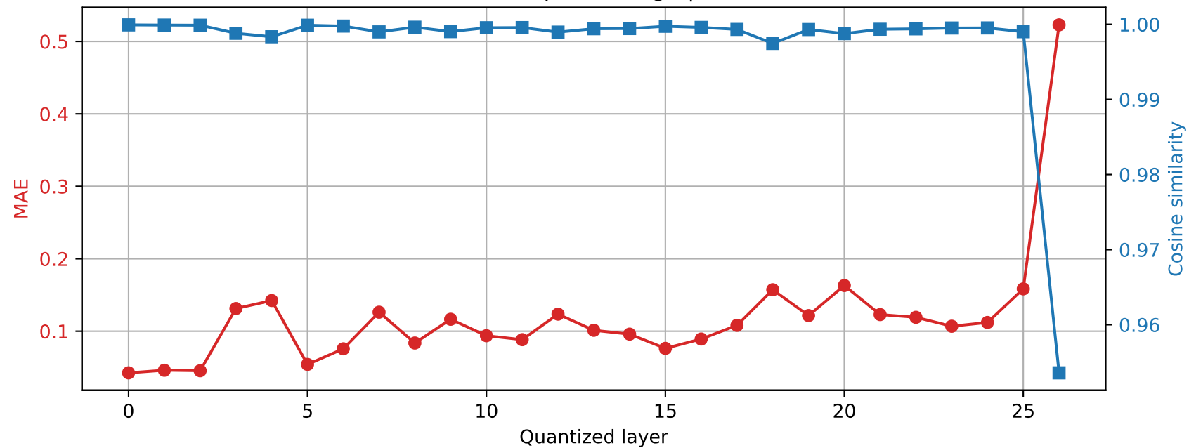
Qwen2.5-7B-Instruct | Prompt 3 Final RMSNorm output damage | float64 → int8
