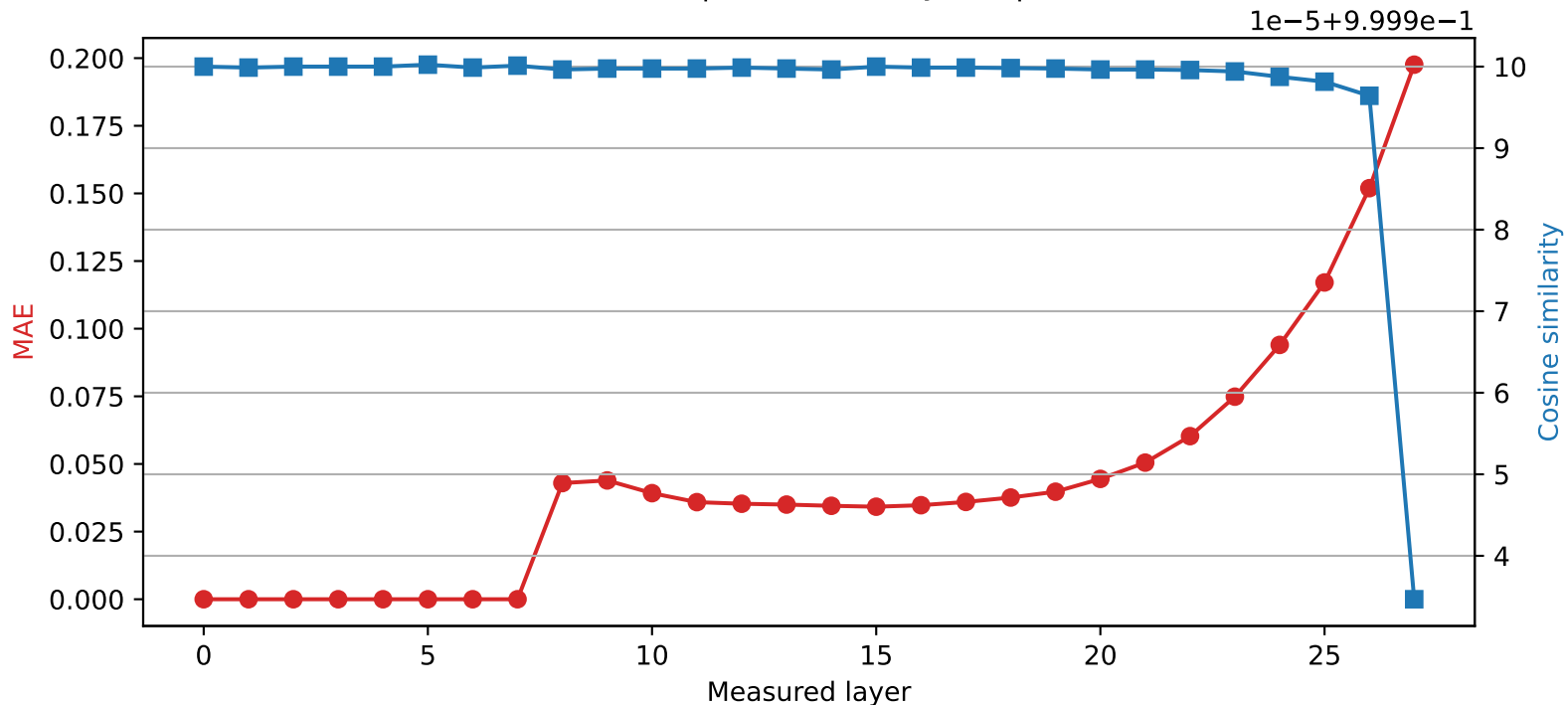
Qwen2.5-7B-Instruct | Quantized layer 7 | float64 → int8
