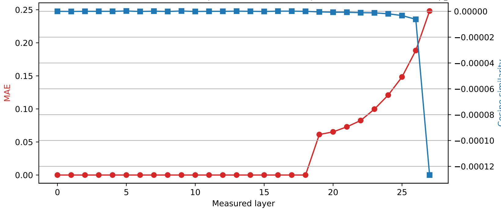
Qwen2.5-7B-Instruct | Quantized layer 18 | float64 → int8
