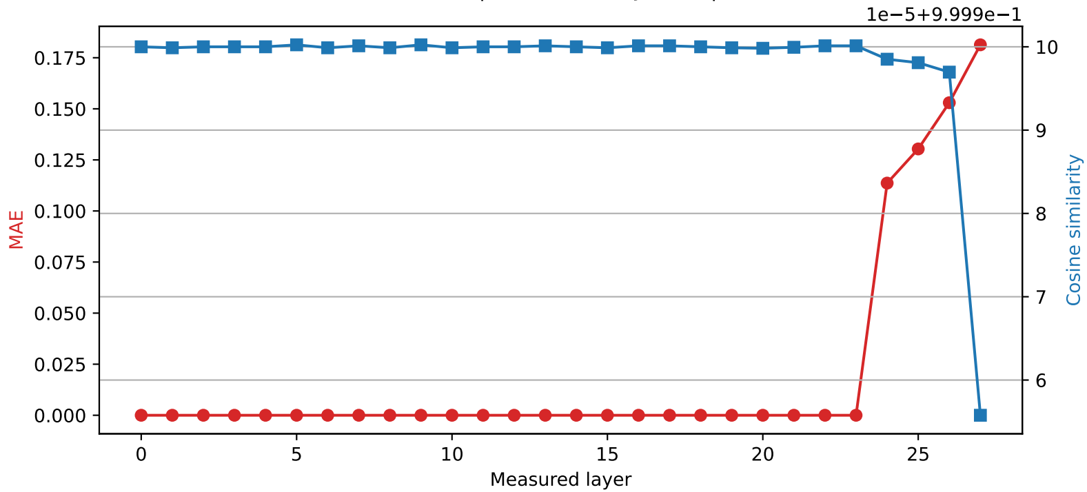
Qwen2.5-7B-Instruct | Quantized layer 23 | float64 \rightarrow int8
