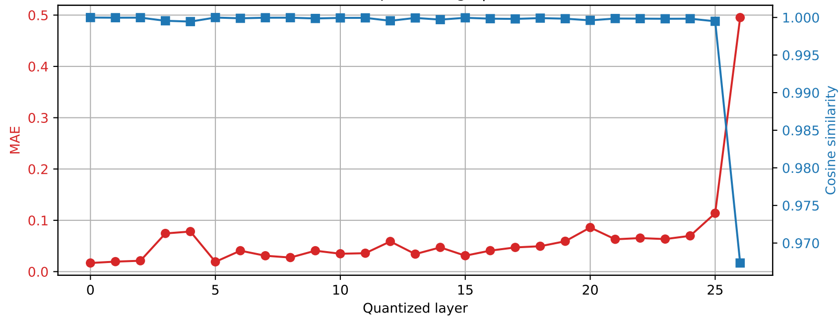
Qwen2.5-7B-Instruct | Prompt 4 Final RMSNorm output damage | float64 \rightarrow int8
