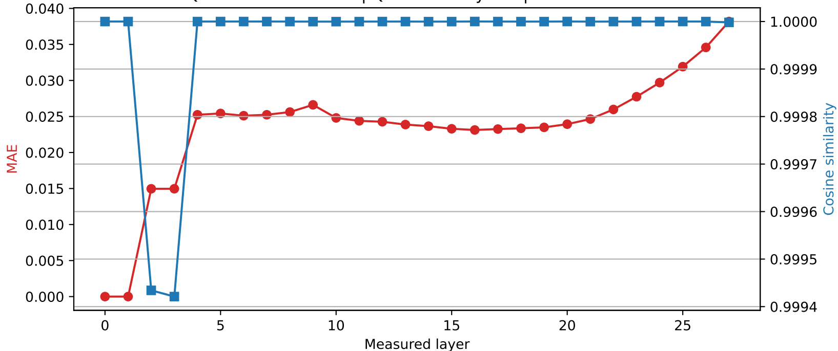
Qwen2.5-7B-Instruct | Quantized layer 1 | float64 → int8
