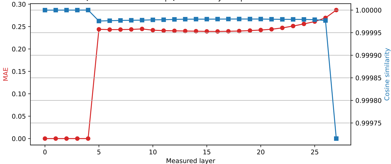
Qwen2.5-7B-Instruct | Quantized layer 4 | float64 → int8
