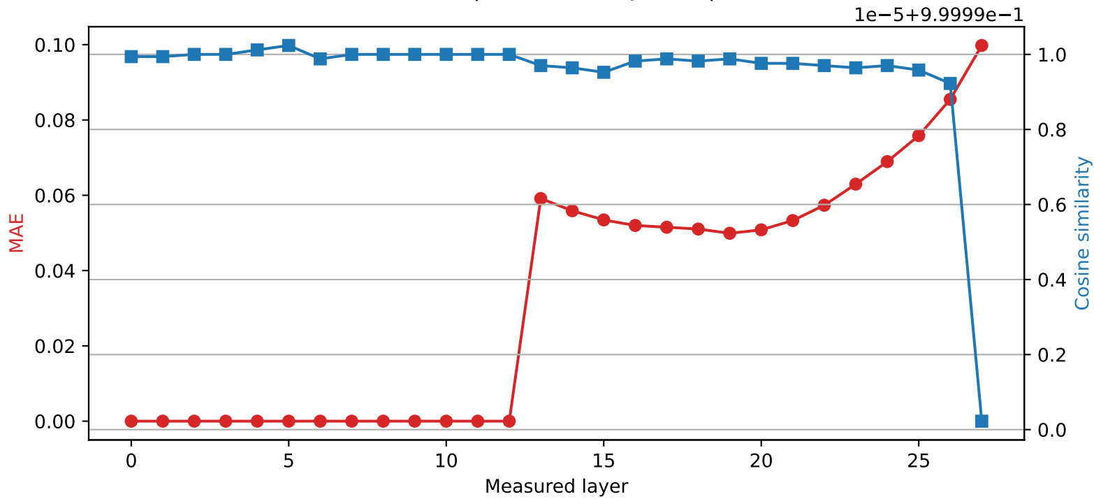
Qwen2.5-7B-Instruct | Quantized layer 12 | float64 → int8
