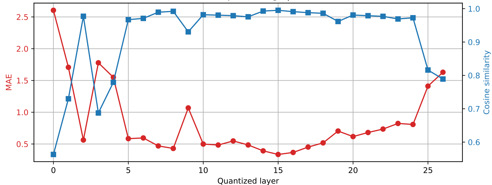
Qwen2.5-7B-Instruct | Prompt 0 Final RMSNorm output damage | float64 \rightarrow int4
