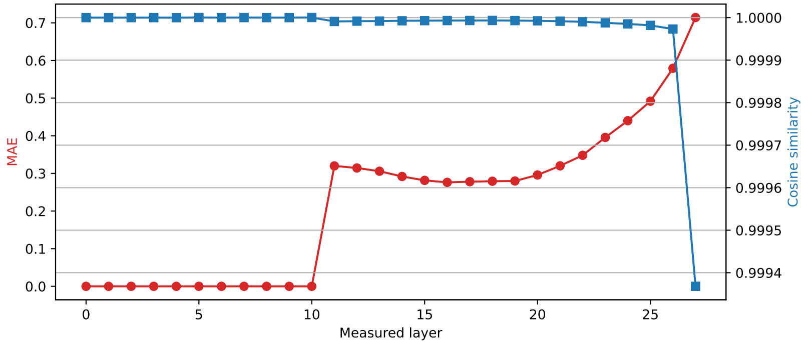
Qwen2.5-7B-Instruct | Quantized layer 10 | float64 \rightarrow int4
