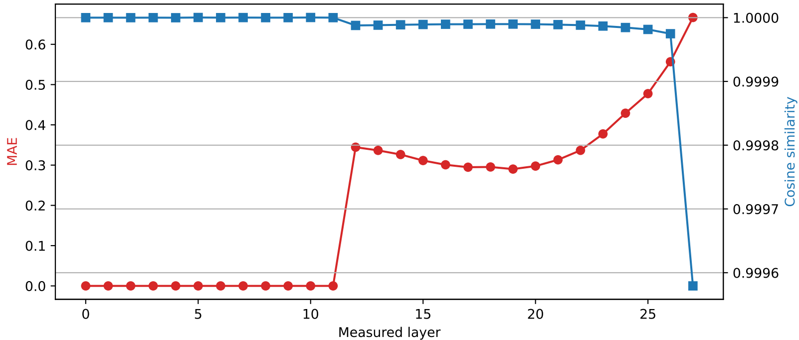
Qwen2.5-7B-Instruct | Quantized layer 11 | float64 → int4
