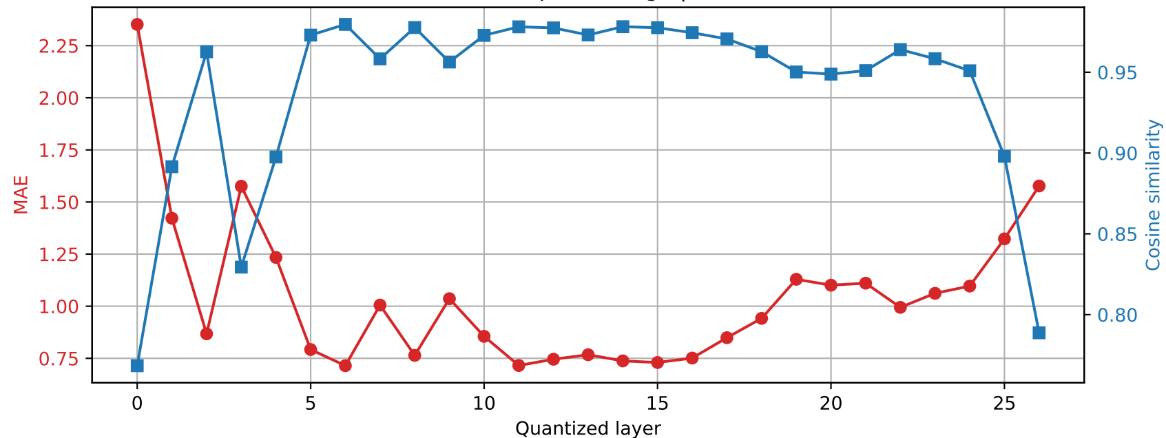
Qwen2.5-7B-Instruct | Prompt 1 Final RMSNorm output damage | float64 \rightarrow int4
