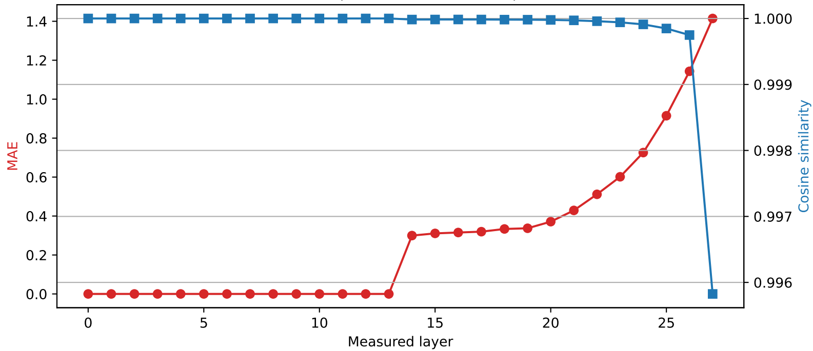
Qwen2.5-7B-Instruct | Quantized layer 13 | float64 \rightarrow int4
