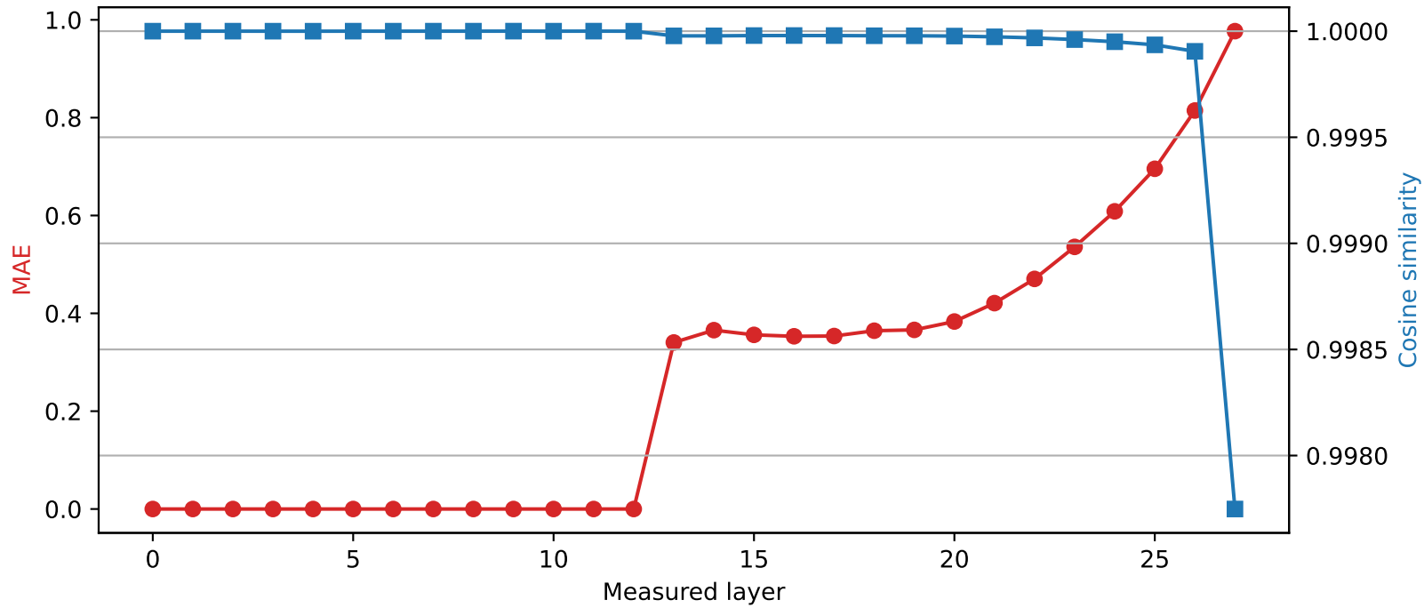
Qwen2.5-7B-Instruct | Quantized layer 12 | float64 \rightarrow int4
