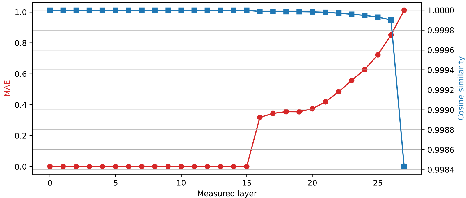
Qwen2.5-7B-Instruct | Quantized layer 15 | float64 → int4
