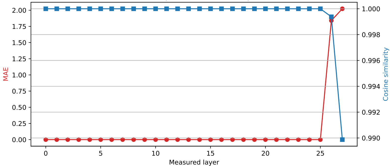
Qwen2.5-7B-Instruct | Quantized layer 25 | float64 → int4
