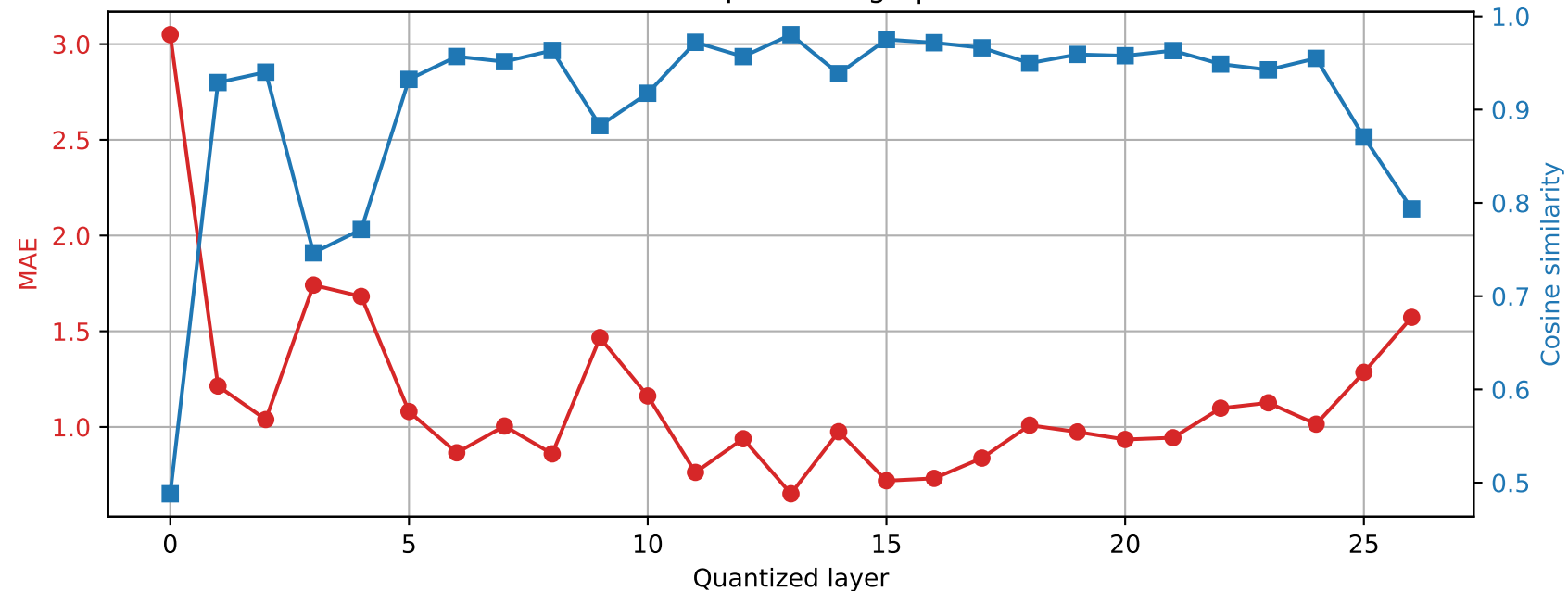
Qwen2.5-7B-Instruct | Prompt 3 Final RMSNorm output damage | float64 \rightarrow int4
