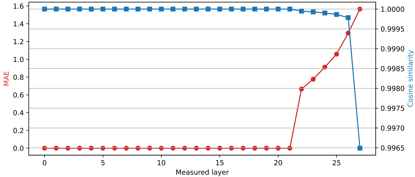
Qwen2.5-7B-Instruct | Quantized layer 21 | float64 → int4
