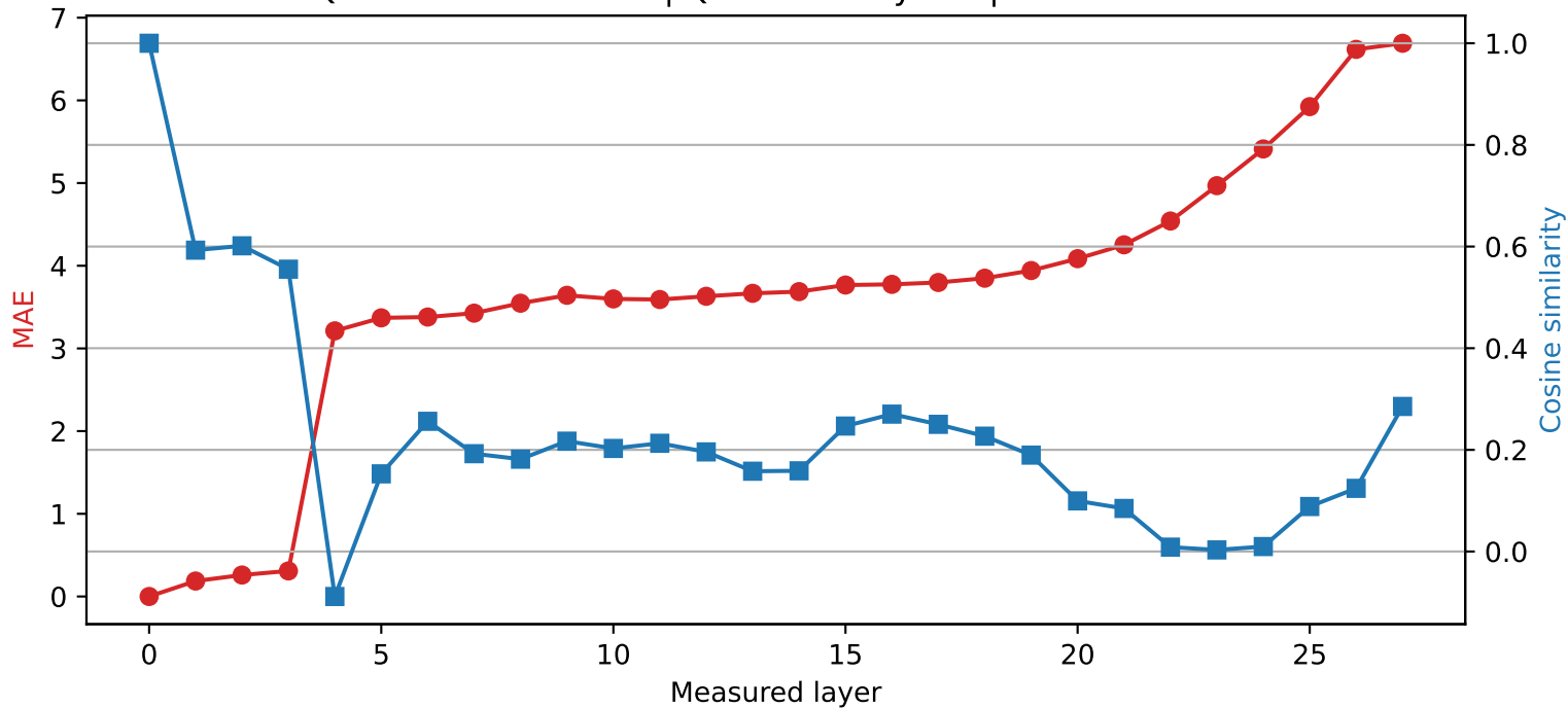
Qwen2.5-7B-Instruct | Quantized layer 0 | float64 → int4
