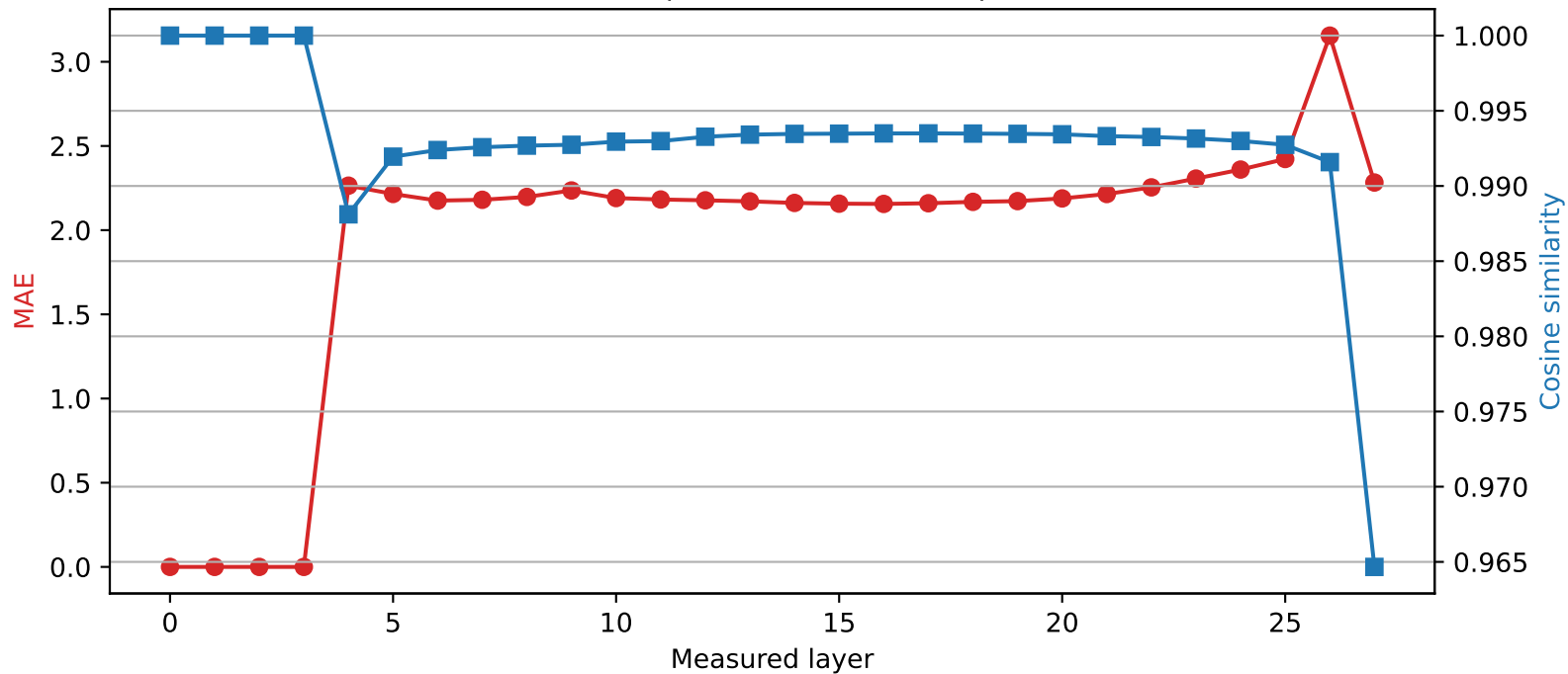
Qwen2.5-7B-Instruct | Quantized layer 3 | float64 → int4
