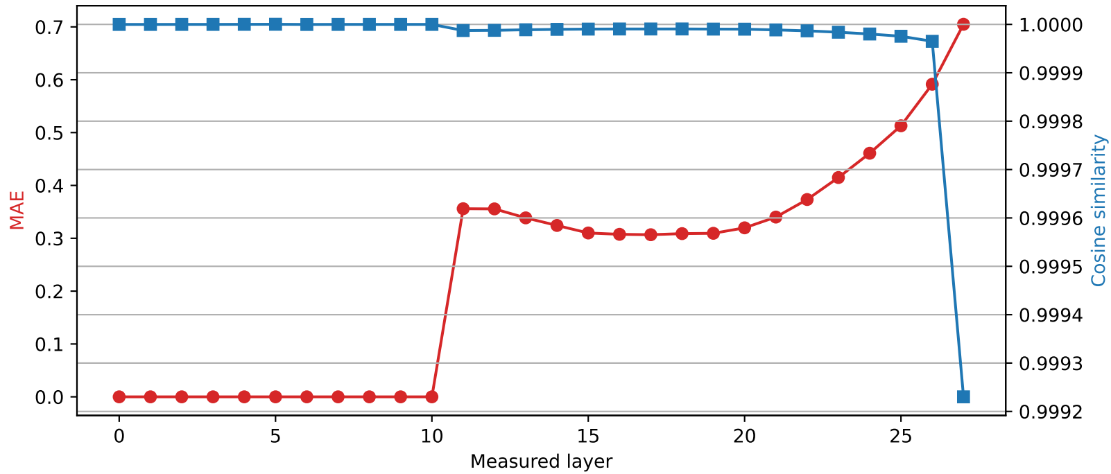
Qwen2.5-7B-Instruct | Quantized layer 10 | float64 → int4
