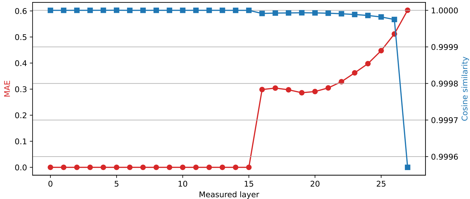
Qwen2.5-7B-Instruct | Quantized layer 15 | float64 \rightarrow int4
