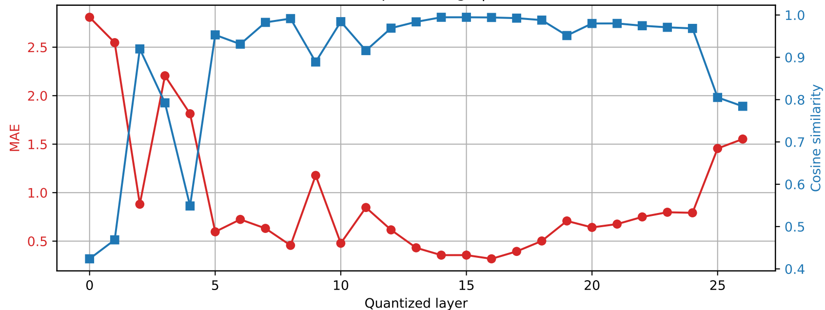
Qwen2.5-7B-Instruct | Prompt 0 Final RMSNorm output damage | float64 \rightarrow int2
