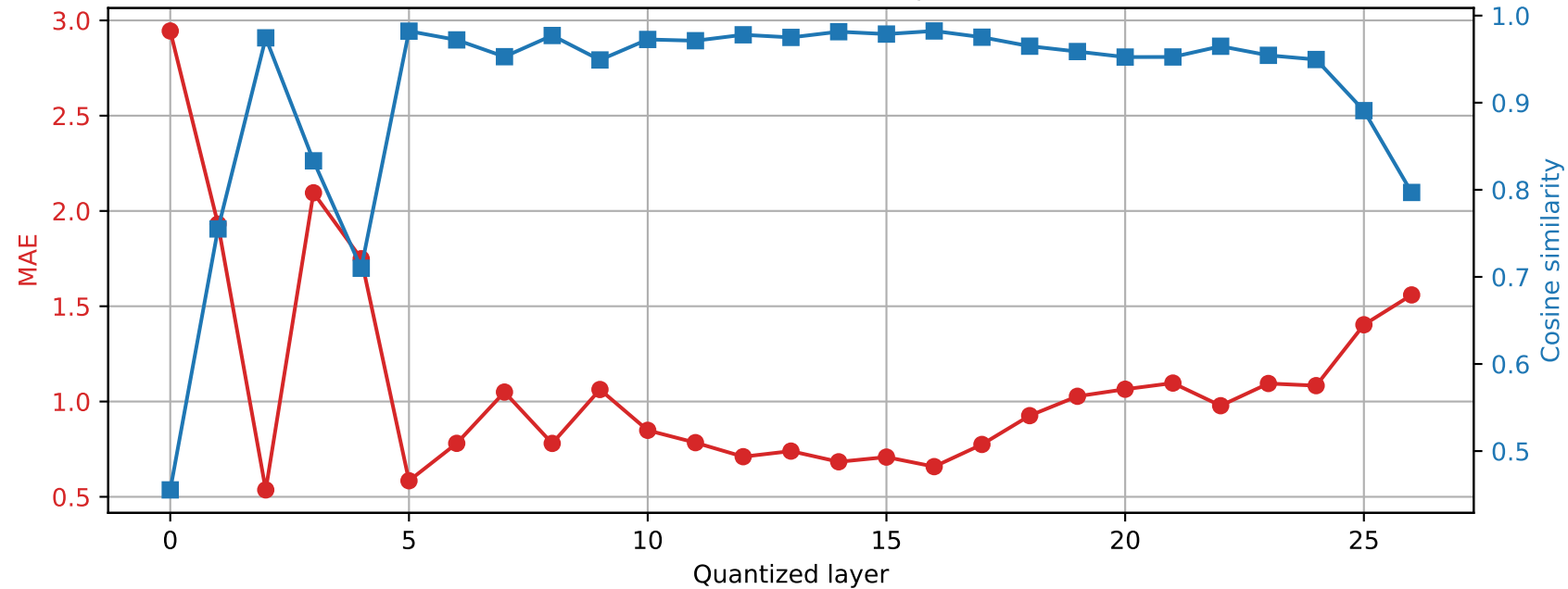
Qwen2.5-7B-Instruct | Prompt 1 Final RMSNorm output damage | float64 \rightarrow int2
